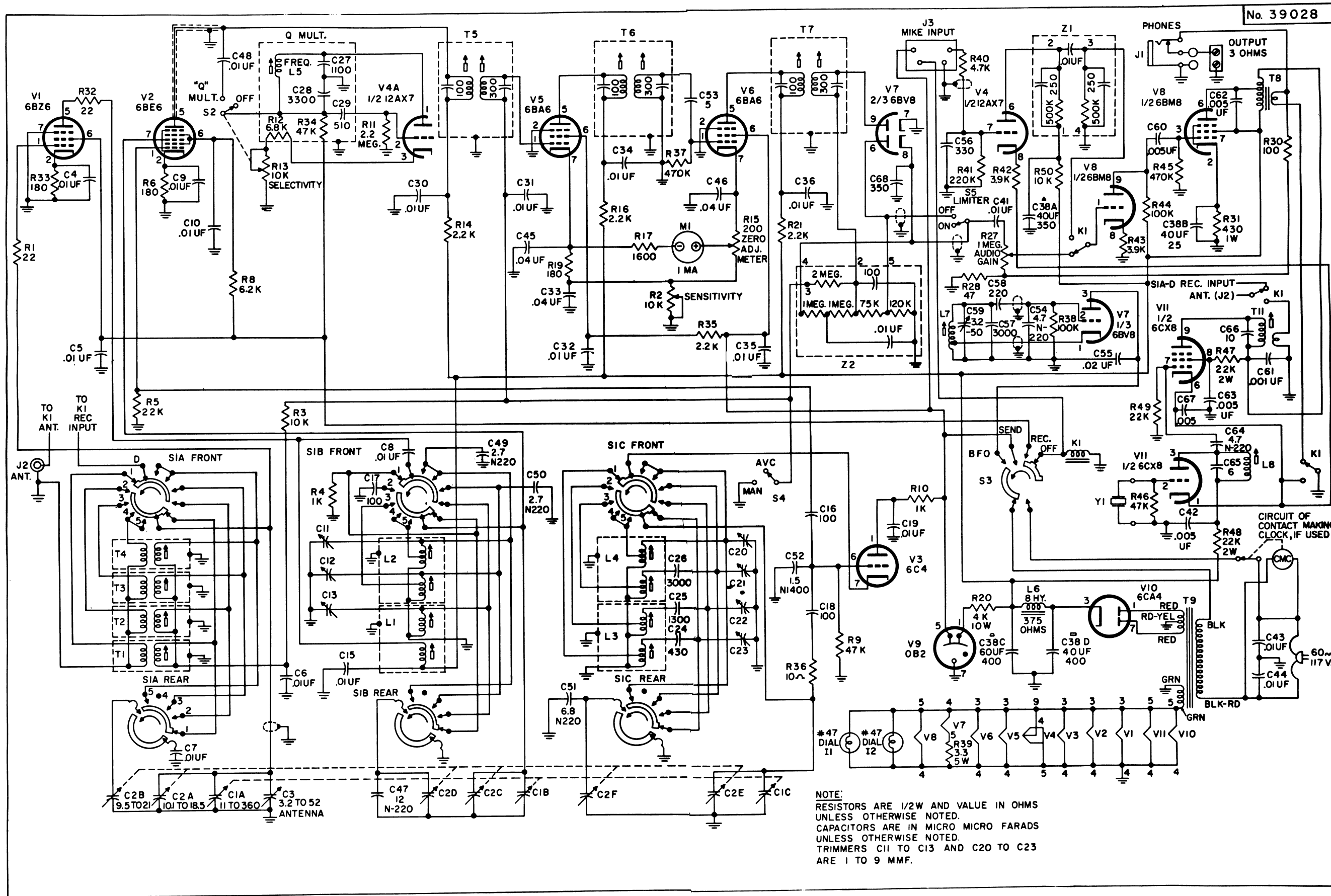
Figure 10. Hammurand HQ-105TR Transceiver Schematic Diagram
