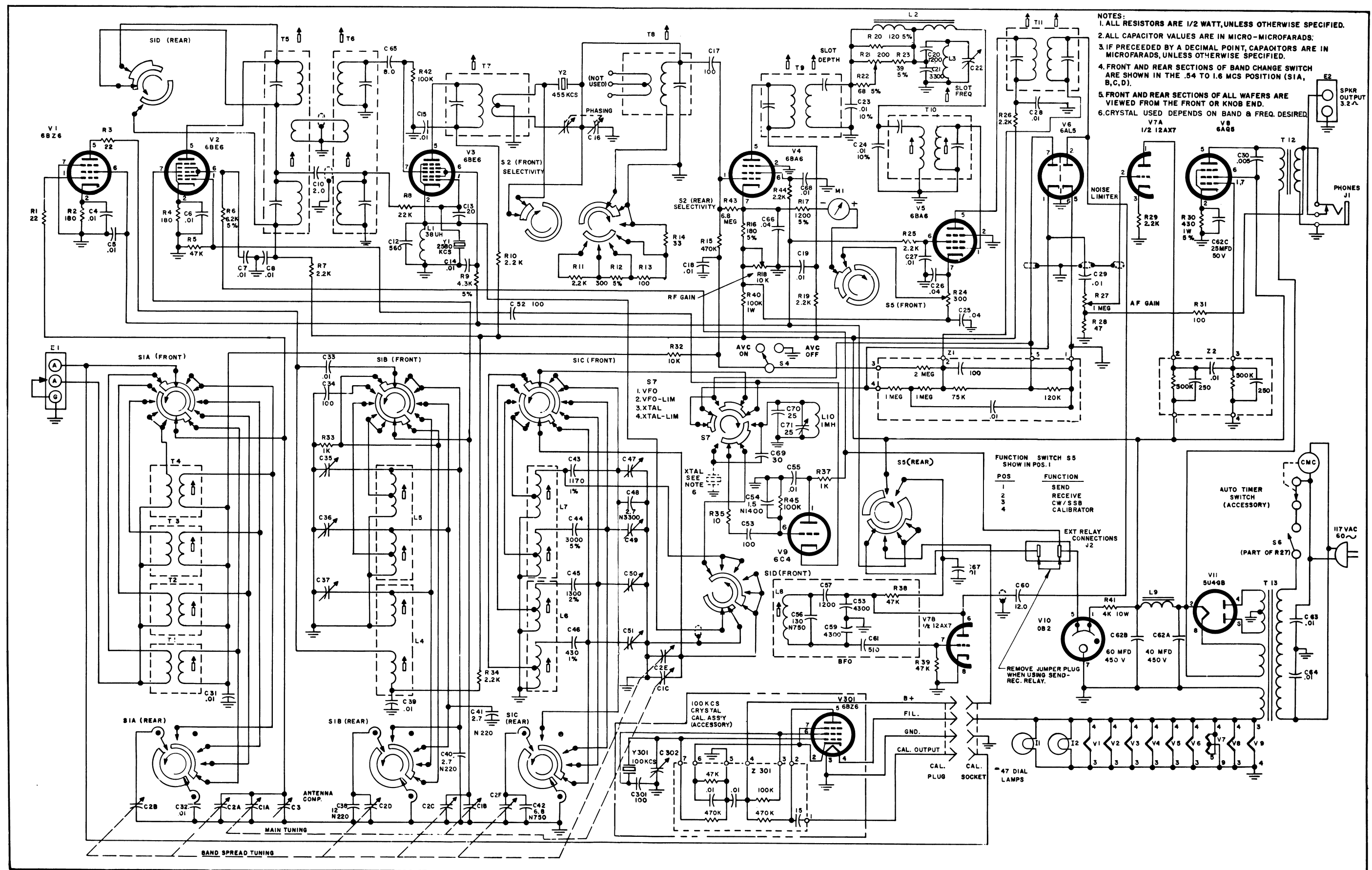
Figure 12. Hammarlund HQ-145X Communications Receiver, Schematic Diagram
