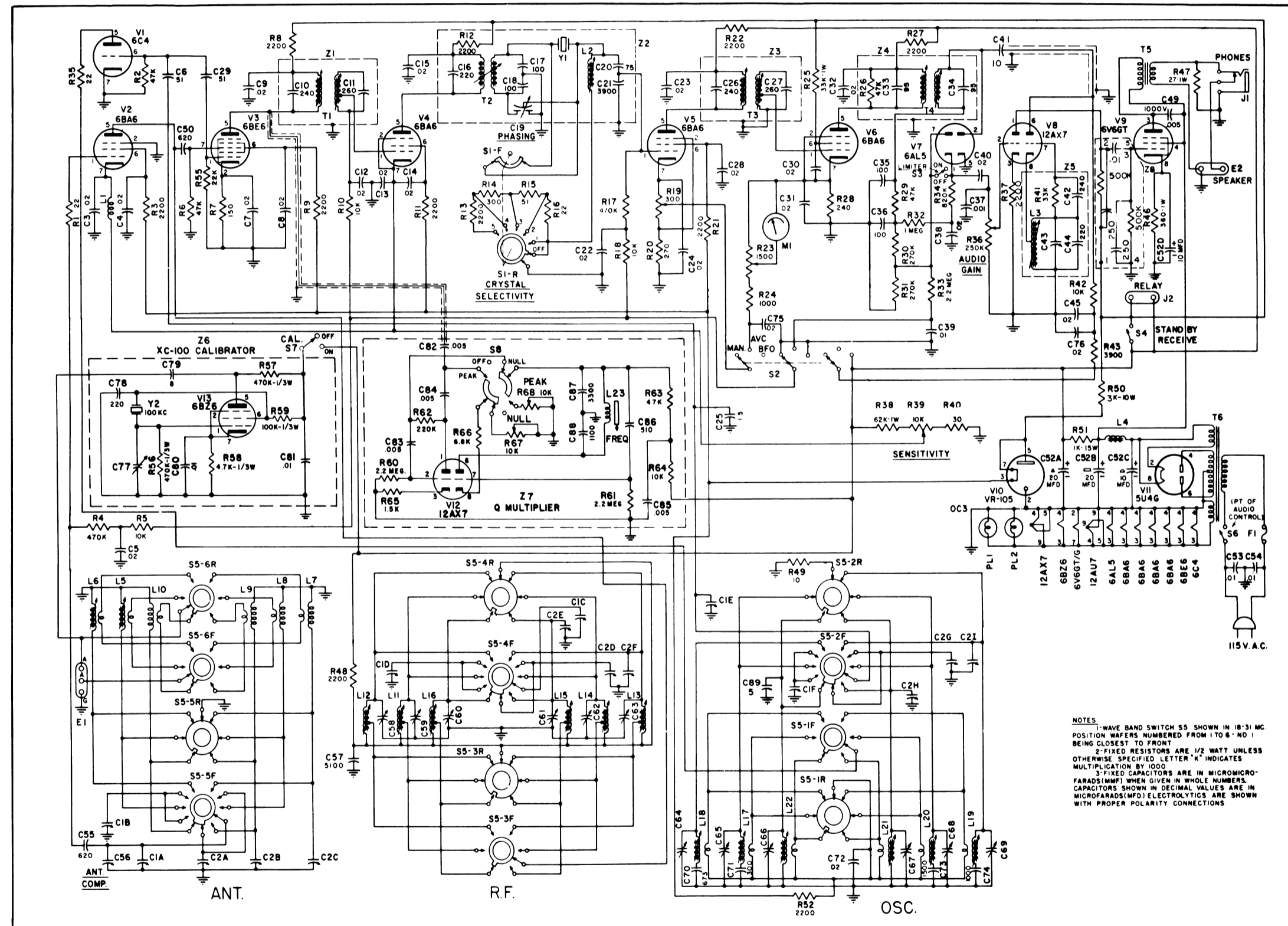
Figure 13. Hammarlund HQ-150 Receiver, Schematic Diagram
