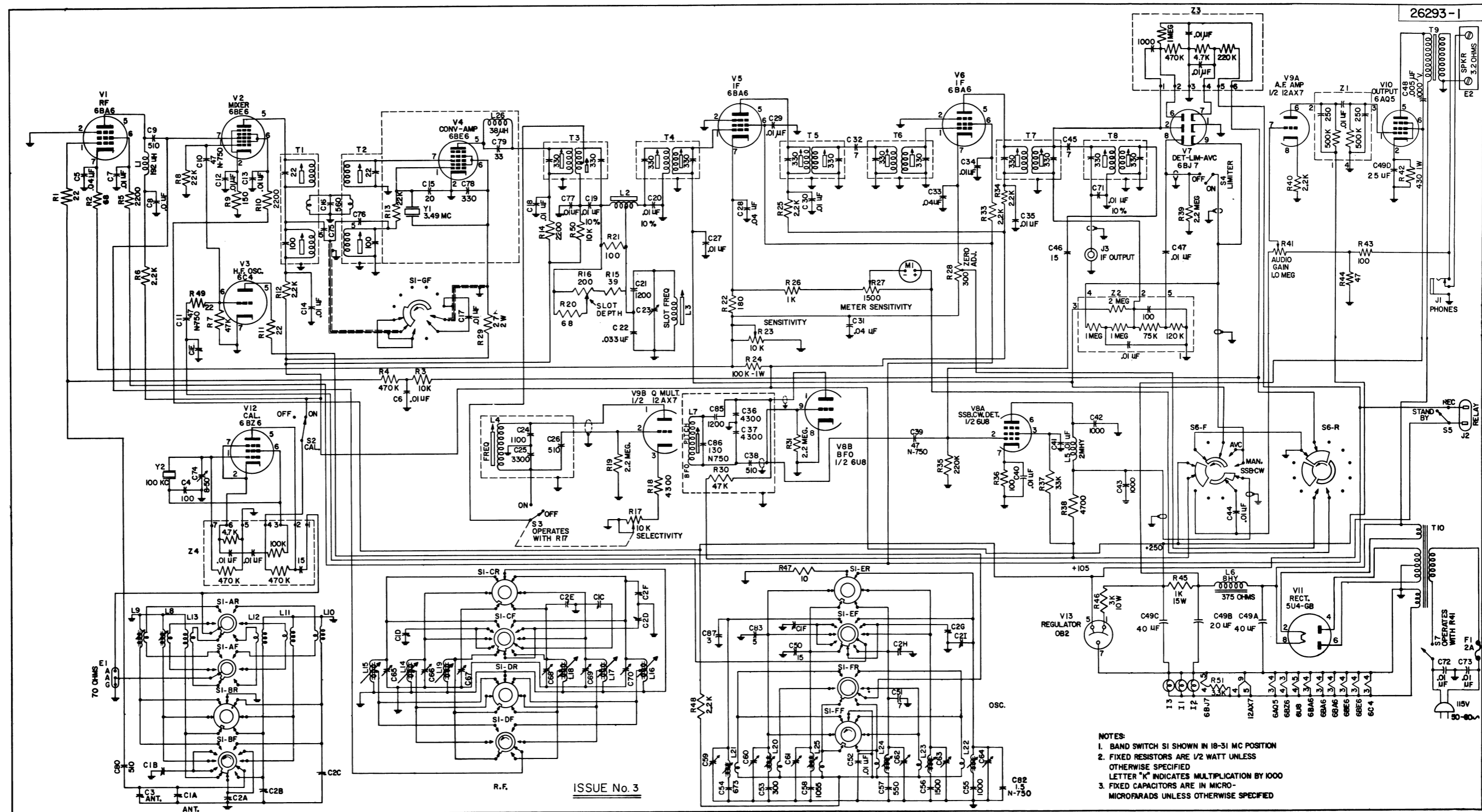
Figure 12. Hammarlund HQ-160 Communications Receiver, Schematic Diagram
