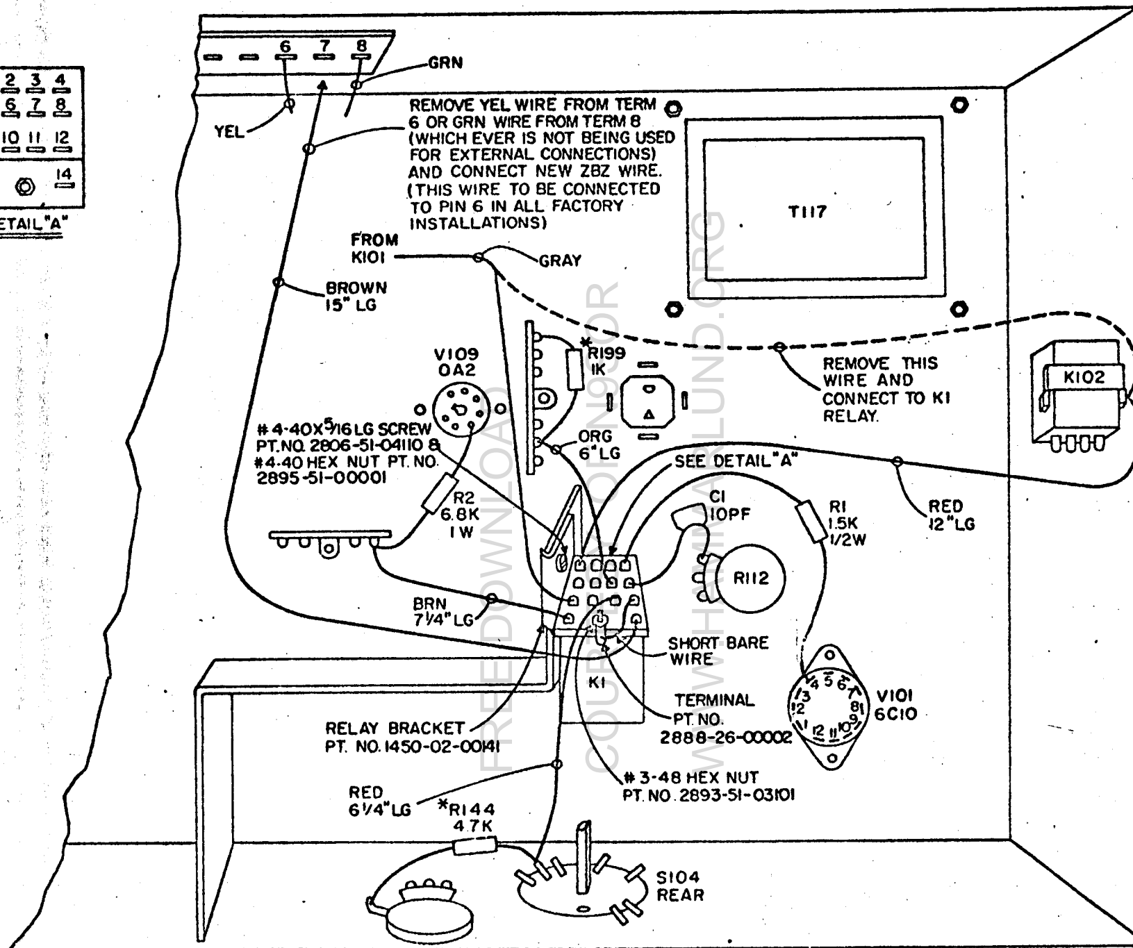
ZBZ INSTALLATION DIAGRAM
