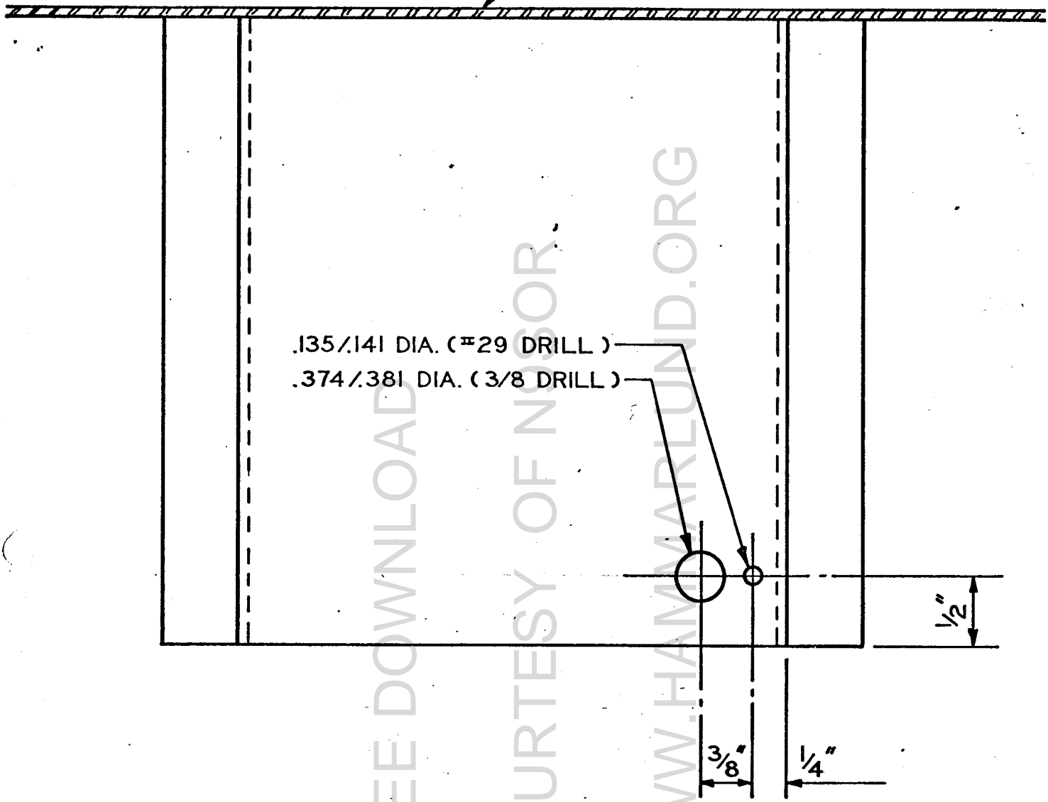
BOTTOM VIEW OF TUBE TRAY SHOWING FIELD DRILLED HOLES CODE 2 MODIFICATION - STEP 12
