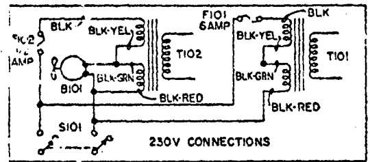
SCHEMATIC DIAGRAM LINEAR AMPLIFIER (HXL-ONE)
